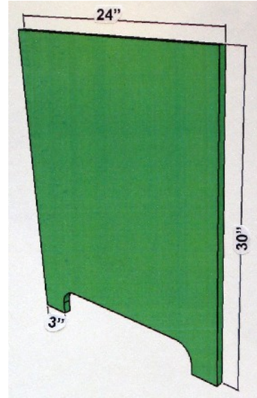
Cut one front panel.
